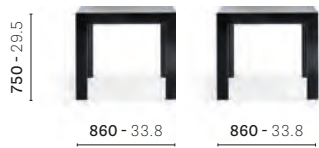
TMF_86X86 Fixed table, aluminium frame, glass top
