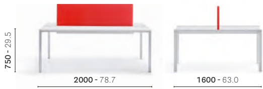
TMS_200X160 2 Work station, aluminium frame, laminate top, setting for divider panel, single cable management (1500x150 - 59.1x5.9)
