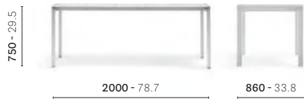
TMD_200X86 Fixed table, aluminium frame and solid laminate top
