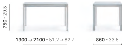
TMA_130X86 Extensible table, aluminium frame, glass or laminate top
